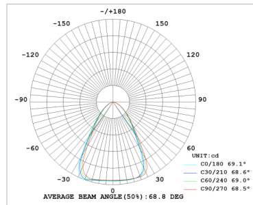
60° PC lens
