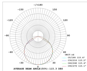
120° PC lens
