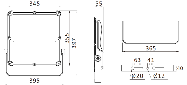
KML-FL200N/KML-FL240N
