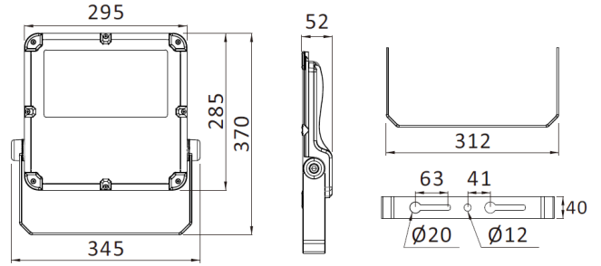
KML-FL100N
