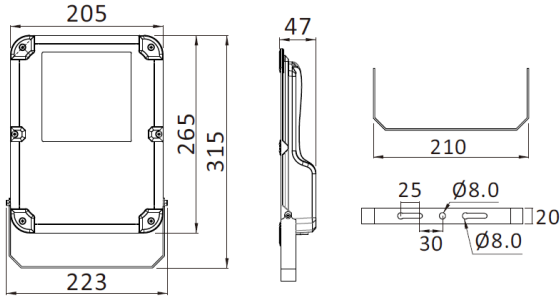
KML-FL050N/KML-FL080N
