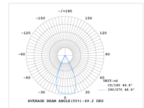
60° PC lens
