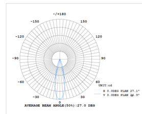
30° PC lens
