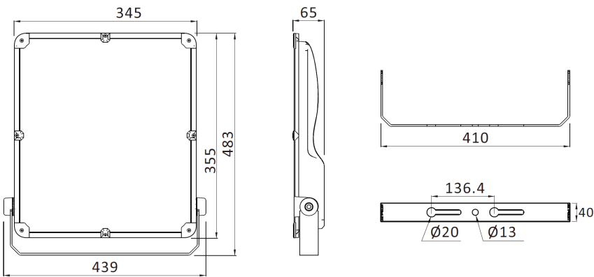
KML-FL300N
