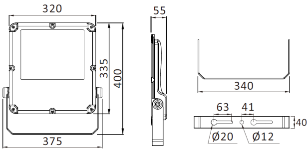
KML-FL150N
